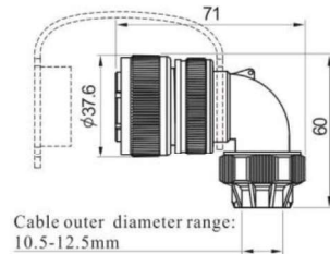
● Cable connector with clamping-nut: TU IP65
