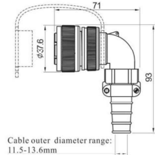
● Cable connector with with rubber sleeve: TV IP65
